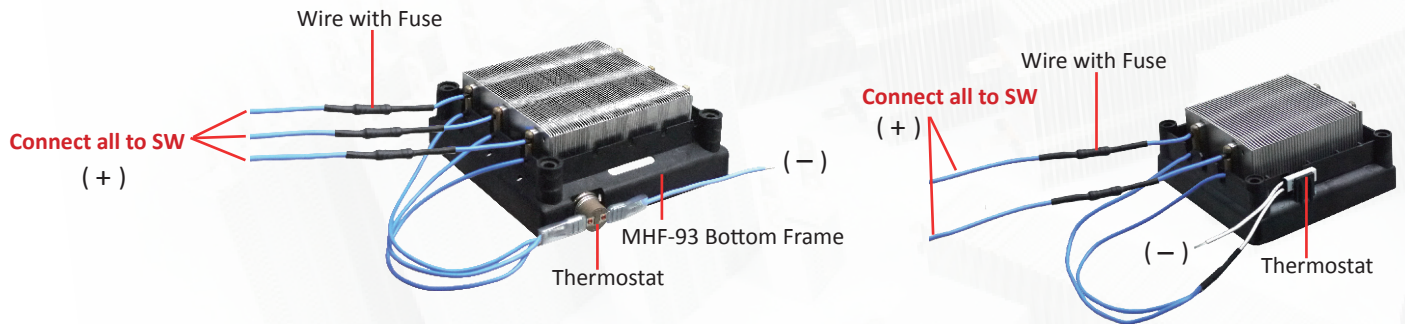
Example 1 – Standard Wiring – Model: MHW-2130S(B/N)-93S(D)4 & SHW-2040M(B)-70S(D)4
